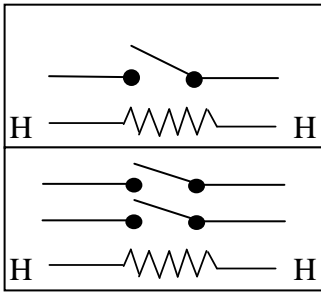
EKS-031 SPST+2SPST Switch
