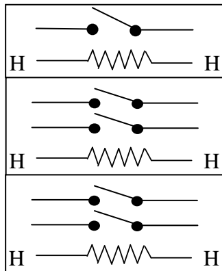
EKS-033 SPST+2SPST+2SPST Switch
