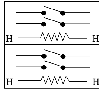
EKS-032 2SPST+2SPST Switch
